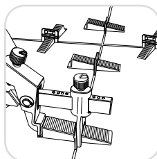
STEP 3 Align pliers and compress until tile is level.
